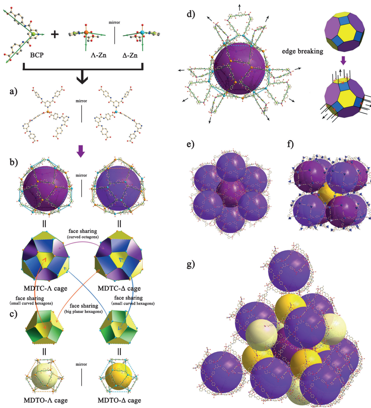
Figure 1. Assembly of NJU-Bai9. a) A pair of enantiotropic Zn centers, each coordinated with three BCP ligands. b) A pair of enantiotropic MDTC cages constructed by 12 \Lambda -Zn centers, 12 \Delta -Zn centers, and 24 ligands centers. c) A pair of enantiotropic MDTO cages abstracted from the space between MDTC cages. The scheme from b to c shows how these four kinds of cages (MDTC- \Lambda , MDTC- \Delta , MDTO- \Lambda , MDTO- \Delta ) are assembled. d) Edge breaking off an MDTC cage, which is illustrated by a regular truncated cuboctahedron. e) Every MDTC- \Lambda cage shares facets with six MDTC- \Delta cages. f) Every MDTO cage shares facets with four MDTC- \Lambda and four MDTC- \Delta cages. g) The overall packing mode of these four kinds of cages.
